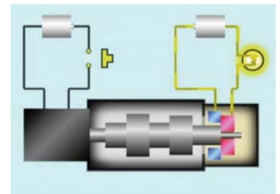
Fig. 1 Solenoid not energized (Switch ON)
